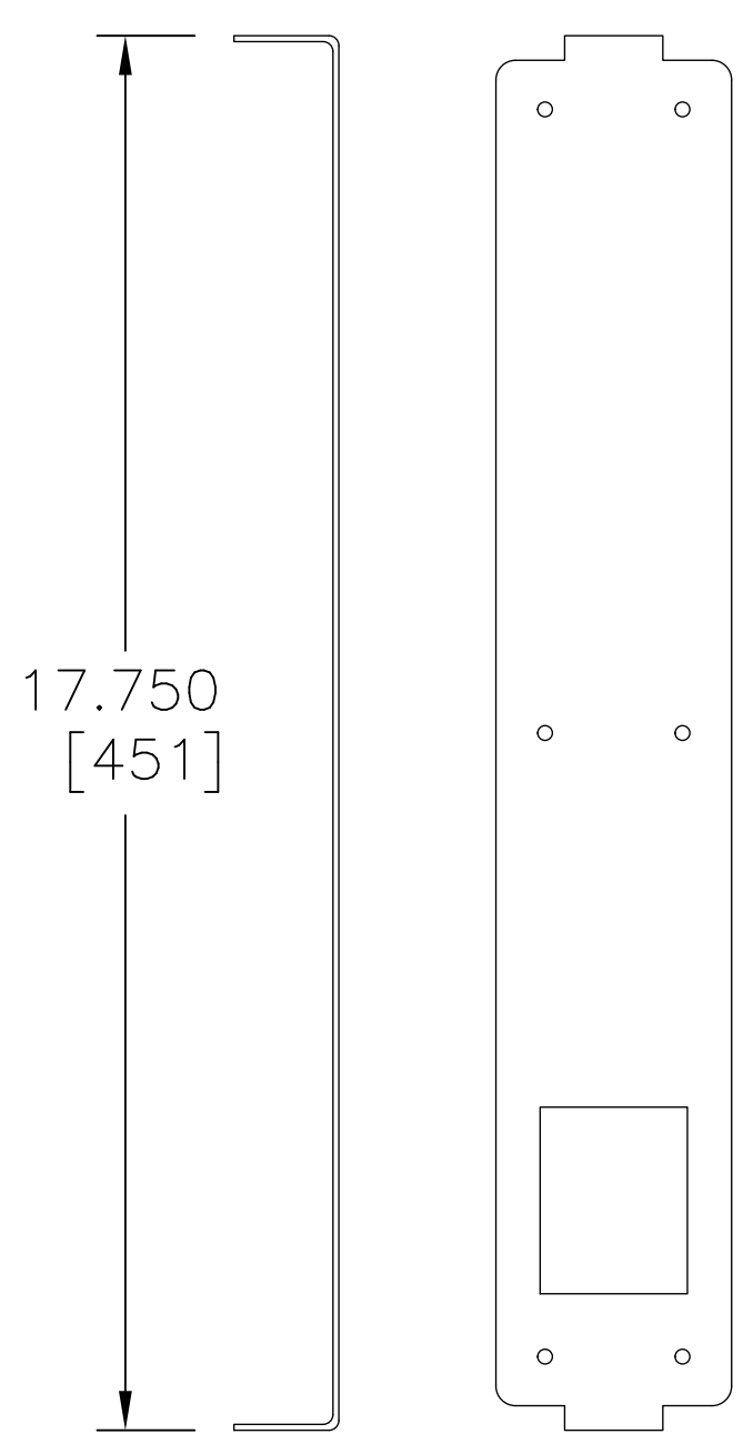
Mounting Bracket
